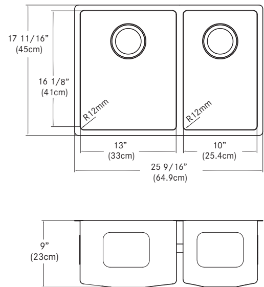
Dimensional Drawing
